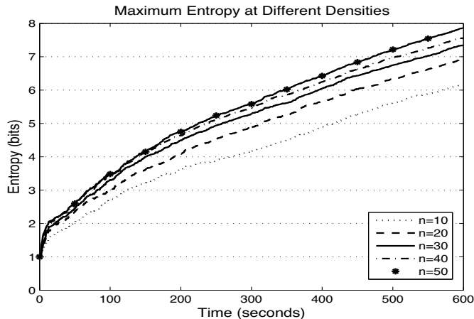
Figure 10: Best-case entropy over time for different user densities.
