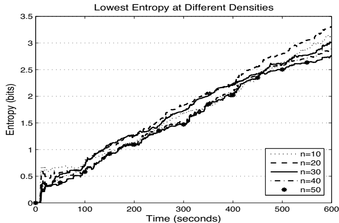
Figure 9: Worst-case entropy over time for different user densities. Around 2.7 bits of entropy achieved even with 10 users.
