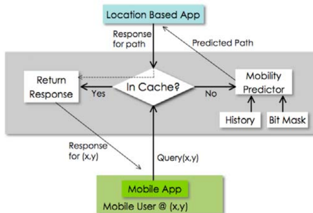
Figure 19: The system diagram for the centralized form of CacheCloak . Mobility prediction based on historical mobility patterns and the bit-mask of caches is performed at the intermediate server. LBS responses for the entire path is cached, and the responses forwarded according to the current (x,y) coordinate of the mobile user.
