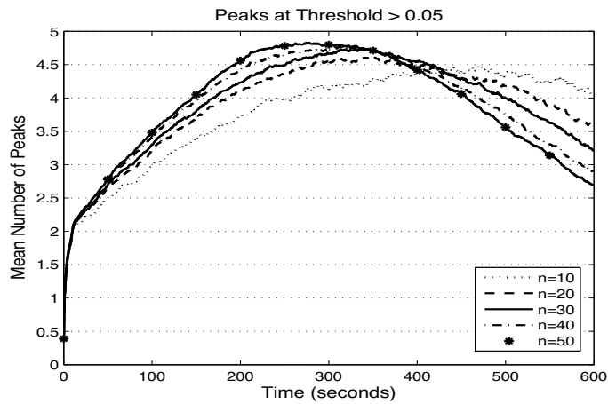
Figure 15: Average number of locations a user might be according to a 0.05 threshold.
