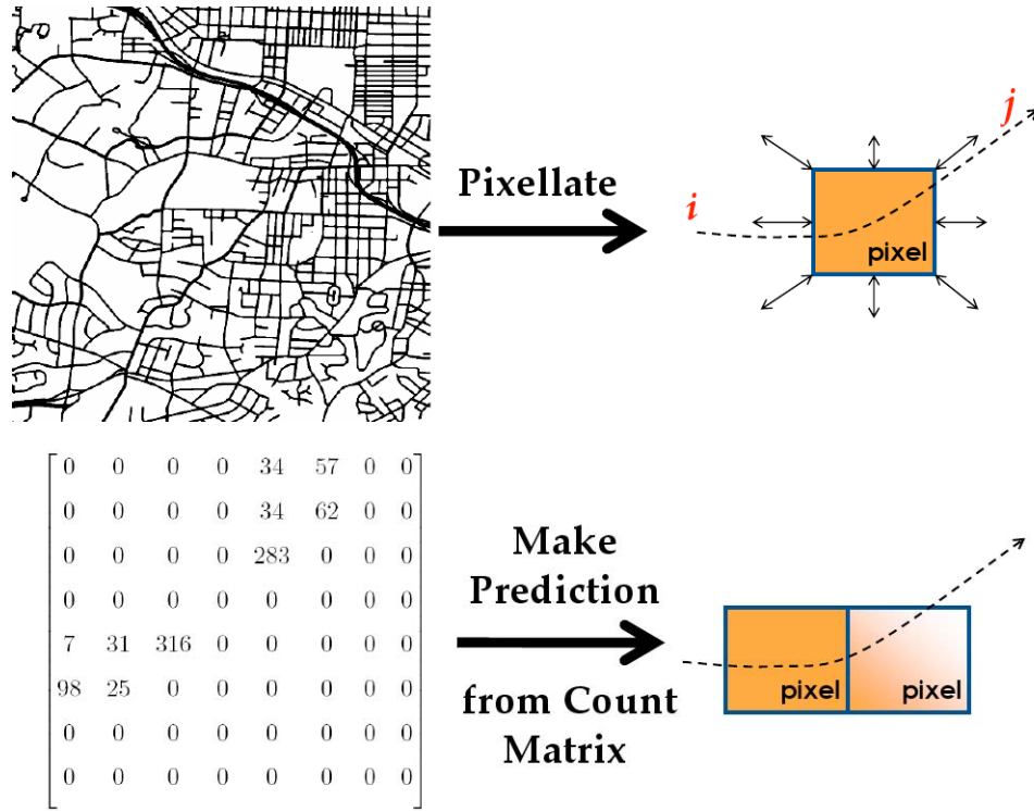
Figure 5: The map of a real city is pixelated, and each pixel is assigned a 8 x 8 count matrix. These count matrices are then used to predict users' paths.
