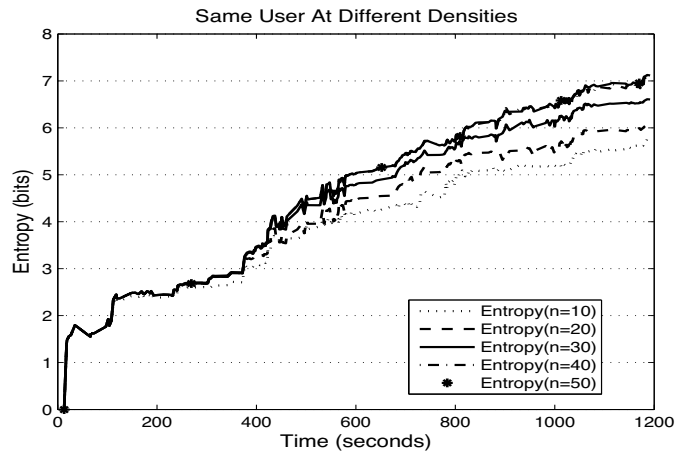
Figure 12: One arbitrary user's entropy over time in different density conditions
