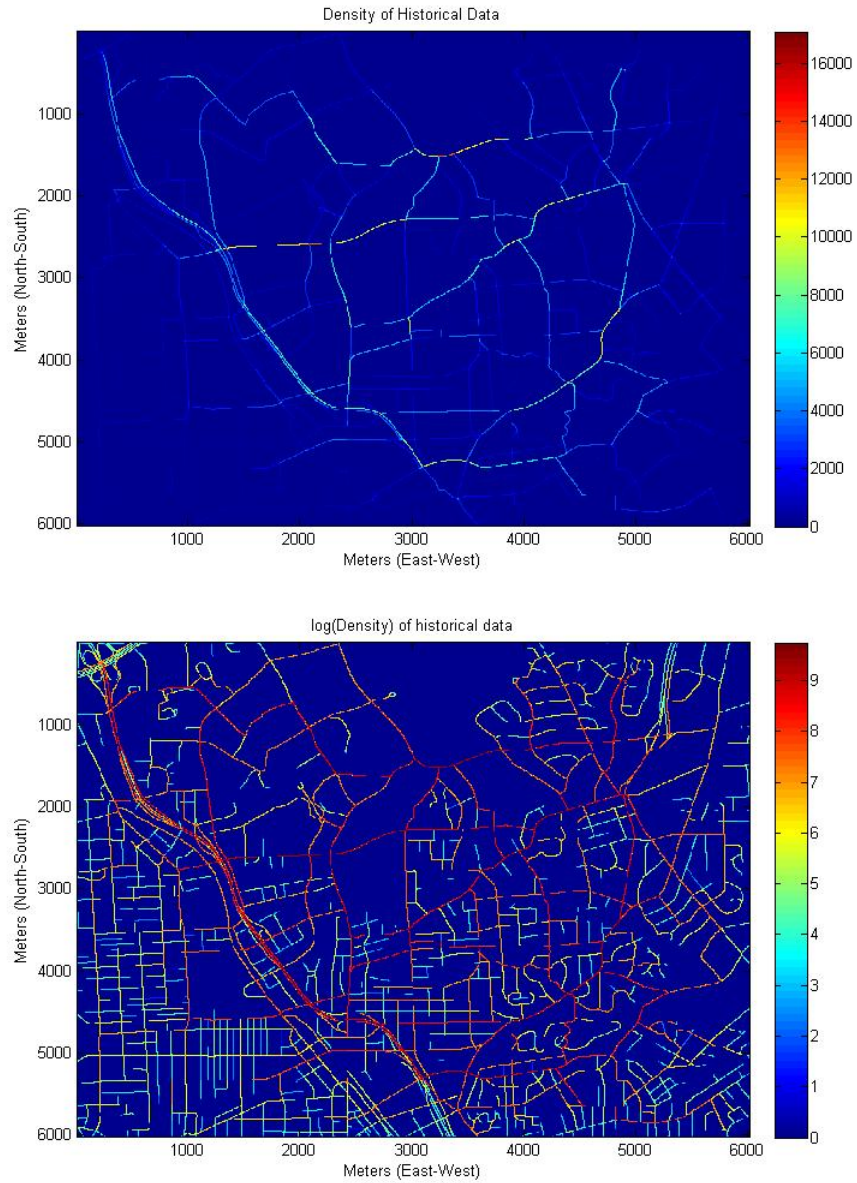
Figure 6: A linear (above) and a logarithmic (below) thermal image of the traffic density generated by VANETMobiSim. Scale bar shows how many users traversed any given pixel on the map.
