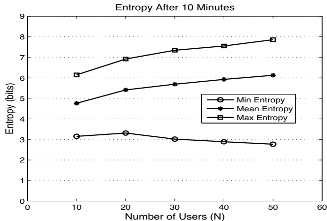
Figure 11: Entropy after 10 minutes of attempted tracking for different user densities.
