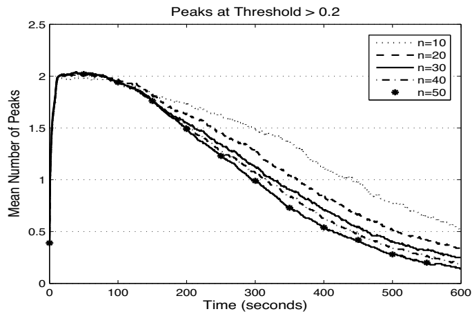
Figure 17: Average number of locations a user might be according to a 0.2 threshold.
