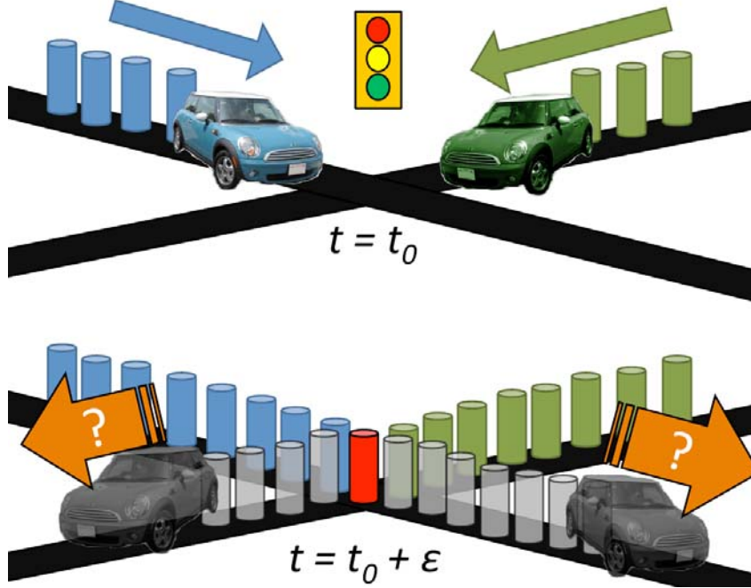
Figure 1: As users move, their locations are relayed to an LBS. Cylinders represent locations where the user has previously revealed a location. An attacker observing the cylinders over time cannot follow two users once they have coincided in space and time. Past the coincidence point, the attacker cannot say whether they turned or went straight.
