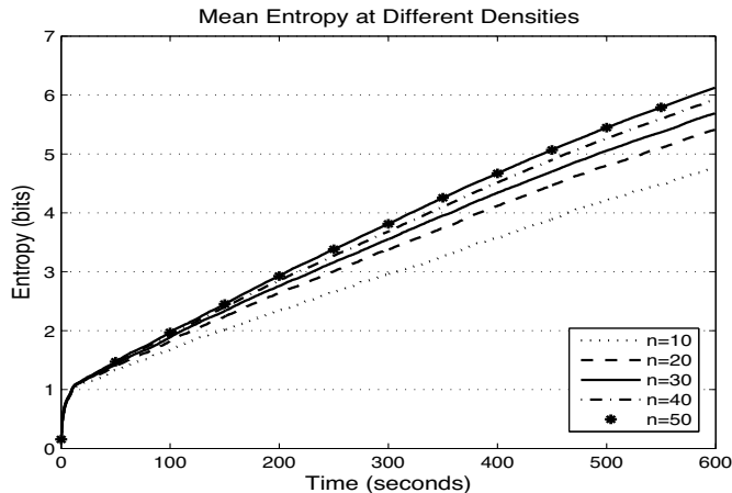
Figure 8: Mean entropy over time for different user densities. Even with 10 to 50 users, the achieved entropy is around 5 bits in 10 minutes (600s). In reality, the number of users are likely to be far greater, resulting in greater entropy.
