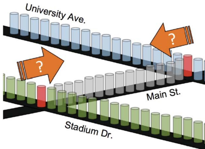
Figure 4: This figure is the view through the eyes of the LBS. The cylinders show locations for which the LBS has received data queries. The LBS cannot determine what triggered the new set of queries along Main Street. It could be users turning in from University Avenue, or from Stadium Drive, or a user coming out into Main Street from her driveway.
