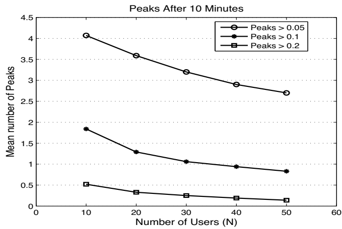
Figure 18: Variation of number of peaks left after 10 minutes at different densities and thresholds. The number of peaks for a given threshold decreases with increasing users, showing that more users offer greater opportunity to hide.
