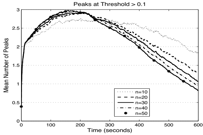
Figure 16: Average number of locations a user might be according to a 0.1 threshold.
