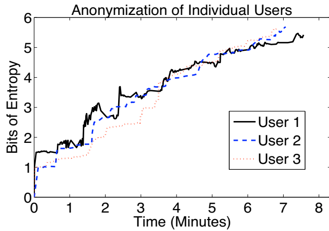
Figure 13: Three arbitrary users' entropies over time ( n = 50 )
